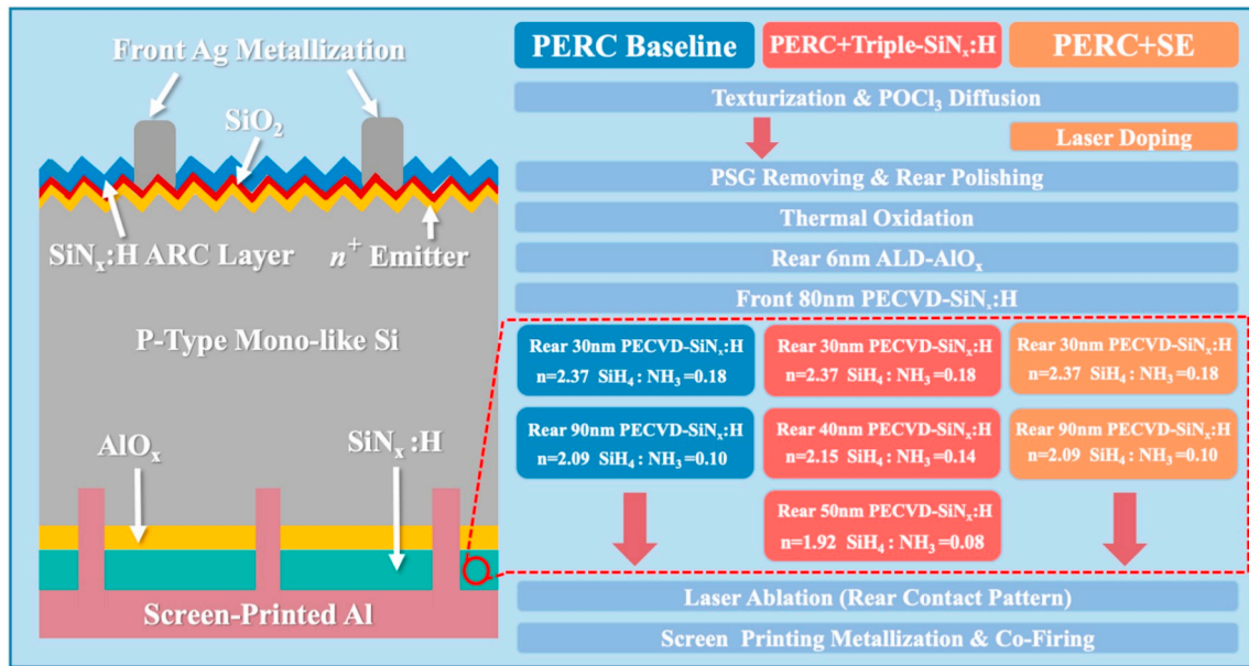
Fig. 1. Schematic of the standard PERC structure (left) and the process flow for the PERC baseline, PERC + Triple-SiN x :H (passivated with triple layers of SiN x :H at the rear side), PERC + SE (combined with SE in the emitter) fabricated in our study together with details of rear AIO x and SiN x :H layers as well as the front SiN x :H ARC layer (right).
