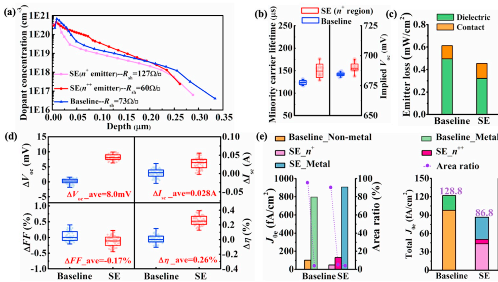
Fig. 5. (a) Phosphorous dopant concentration profiles of the emitters for baseline and SE samples. (b) Measured \tau_{\text{eff}} and implied V_{\text{oc}} for baseline and the n^+ emitter of SE at an injection level of 10^{15}\text{cm}^{-3} with a symmetric structure. (c) Simulated efficiency loss in the emitter for baseline and SE. (d) Measured I - V parameters (relative value of I_{\text{sc}} , V_{\text{oc}} , FF and \eta compared with baseline). (e) Measured J_{0e} of different regions (metal and non-metal for baseline and n^+ emitter, n^{++} emitter and metal for SE) together with the area ratio of the corresponding regions (left), the calculated total J_{0e} as a function of J_{0e} of each region and the corresponding area ratio (right).
