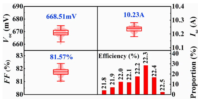
Fig. 6. Measured I - V parameters (absolute values of V_{oc} , I_{sc} , FF and \eta of mono-like PERCs combined with triple- \text{SiN}_x\text{:H} , rear contact pattern of L^R/L = 34.4\% and SE technology).
